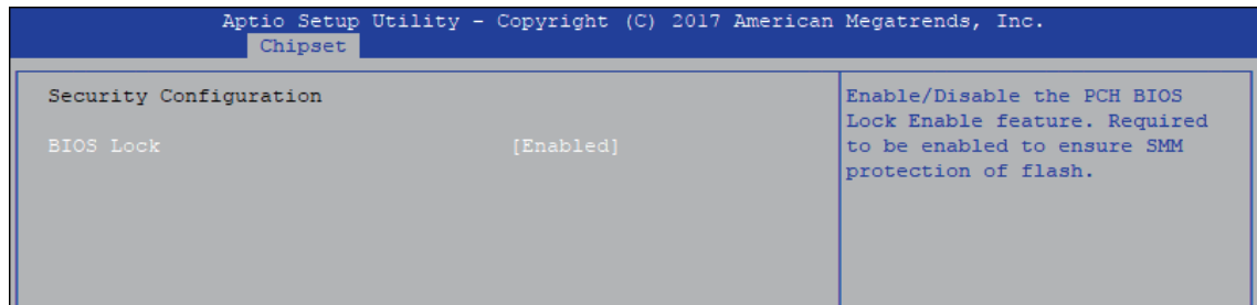
Figure 4-4-2-3 : Security Settings
